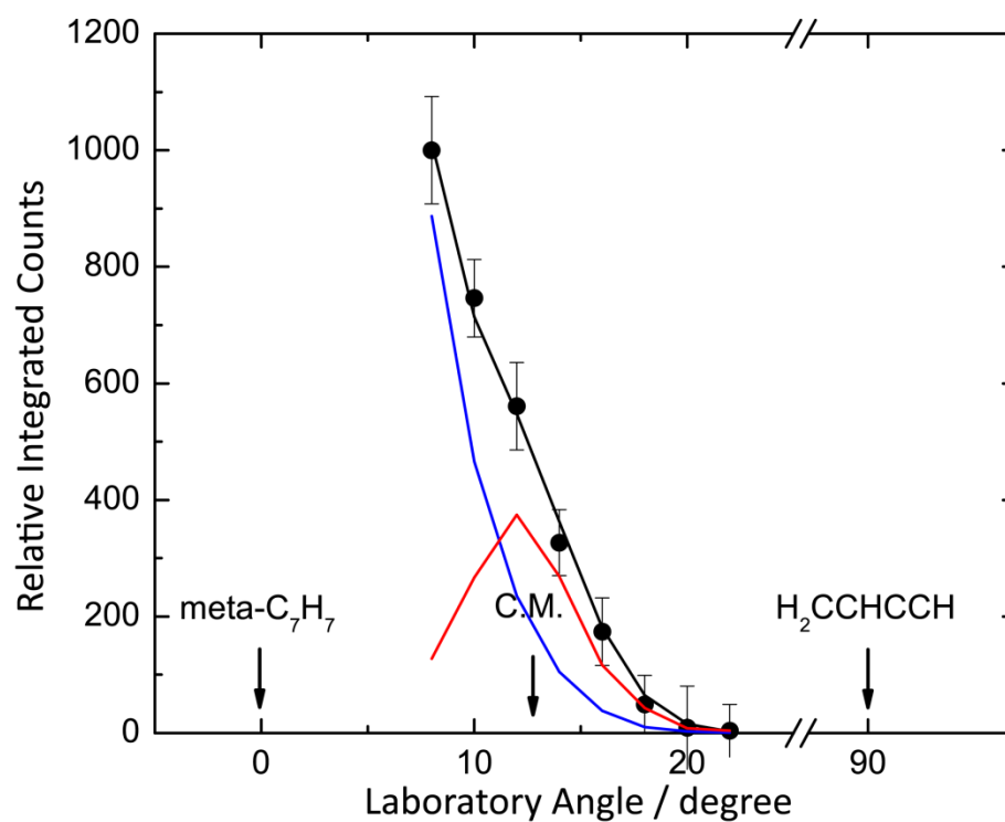
Figure 3. Laboratory angular distribution for the reaction of meta-tolyl with vinylacetylene recorded at mass-to-charge ratio ( m/z ) of 142. The solid circles present the experimental data, the red and blue lines represent the fit for the reactive and non-reactive scattering channel, respectively. The black solid lines represent the overall fit.
