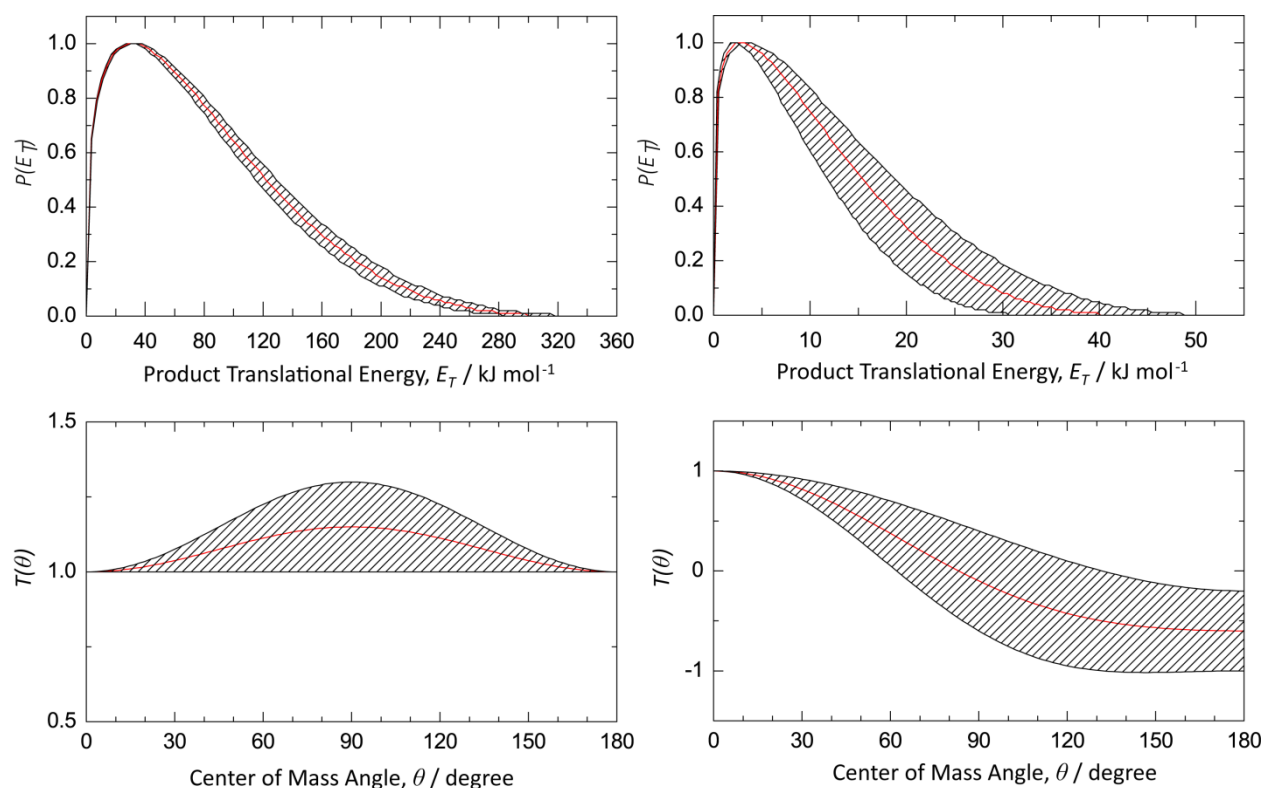
Figure 4. Center-of-mass translational energy distributions P(E_T) s (top) and angular distributions T(\theta) s (bottom) in the reaction of meta-tolyl with vinylacetylene in the reactive scattering channel (left column) and the non-reactive scattering channel (right column), respectively. The hatched areas account for fits within the experimental error limits.
