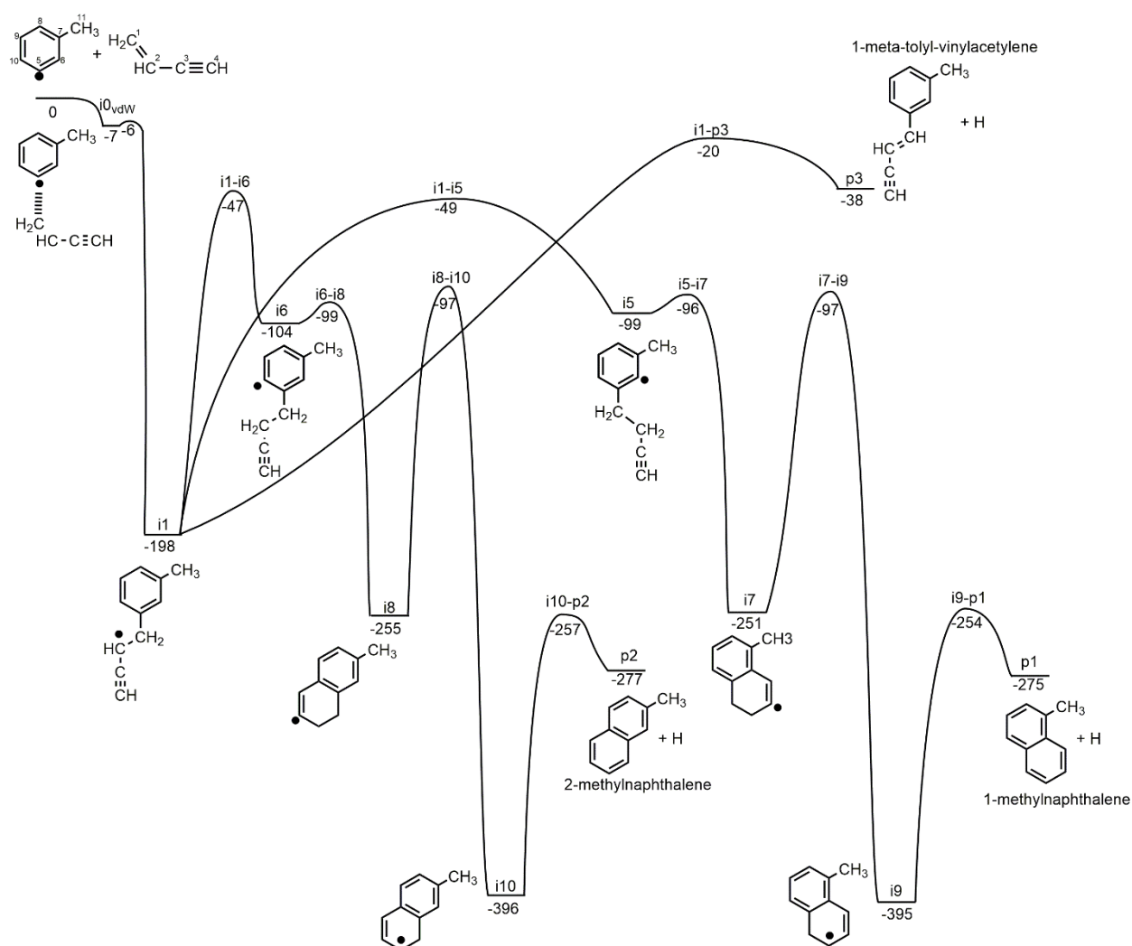
Figure 5. Proposed reaction mechanism based on stationary points on the C_{11}H_{11} potential energy surface for the reaction of the meta-tolyl radical with C1 carbon of vinylacetylene. Energies for intermediates, transition states, and products are given relative to the reactants energy (in \text{kJ mol}^{-1} ) at the at the UCCSD(T)-F12b/cc-pVDZ//UM06-2x/cc-pVTZ + ZPE(UM06-2x/cc-pVTZ) level of theory.
