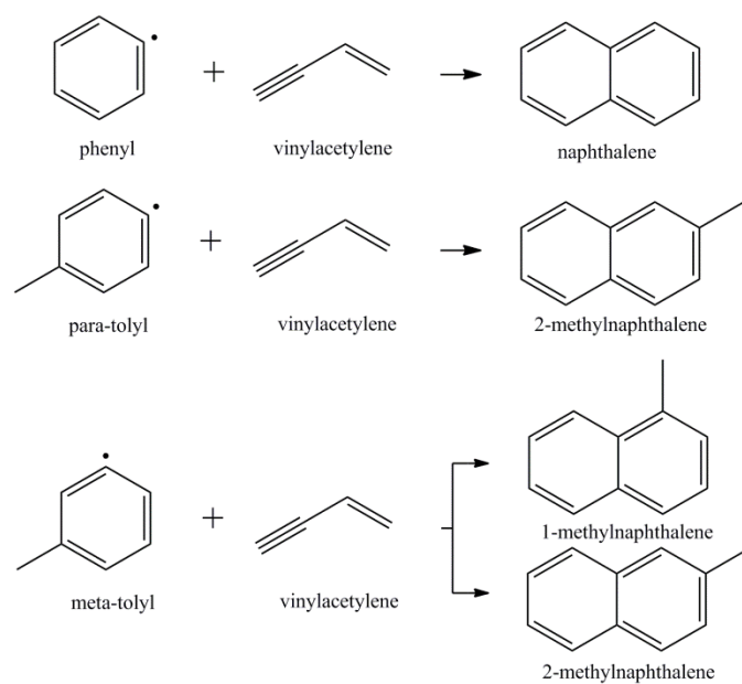
Figure 1. Formation of (methyl-)naphthalenes via the crossed beam reactions of phenyl-type radicals (phenyl, para-tolyl, meta-tolyl) with vinylacetylene.
