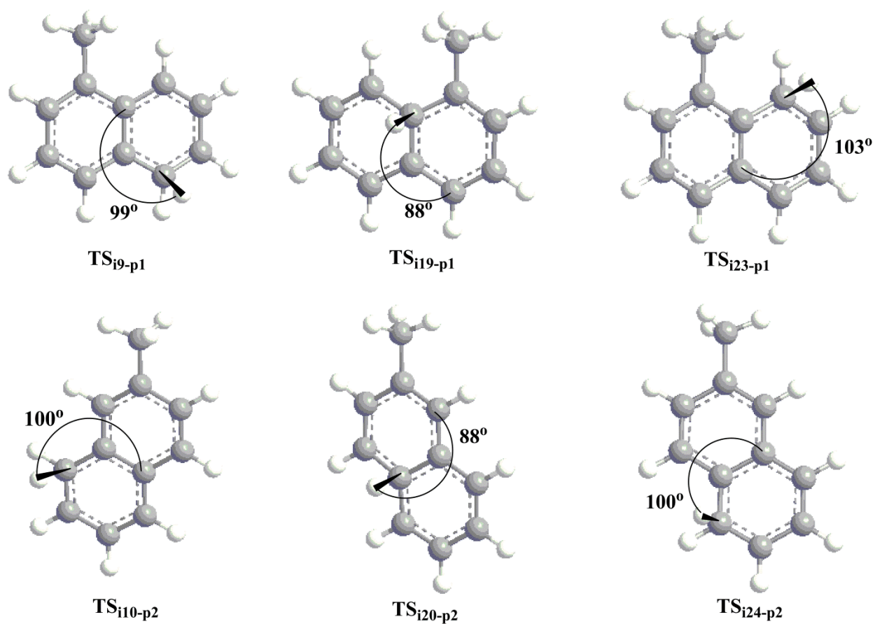
Figure 9. Computed dihedral angle between the molecular plane of the nascent 1-methylnaphthalene (top) and 2-methylnaphthalene (bottom) and dissociating H atom at the transition states from the intermediates i9 , i19 , and i23 (top) to i10 , i20 , and i24 (bottom).
