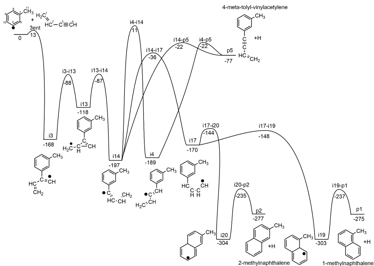
Figure 7. Proposed reaction mechanism based on stationary points on the C_{11}H_{11} potential energy surface for the reaction of the meta-tolyl radical with C3 carbon of vinylacetylene. Energies for intermediates, transition states, and products are given relative to the reactants energy (in \text{kJ mol}^{-1} ) at the at the UCCSD(T)-F12b/cc-pVDZ//UM06-2x/cc-pVTZ + ZPE(UM06-2x/cc-pVTZ) level of theory.
