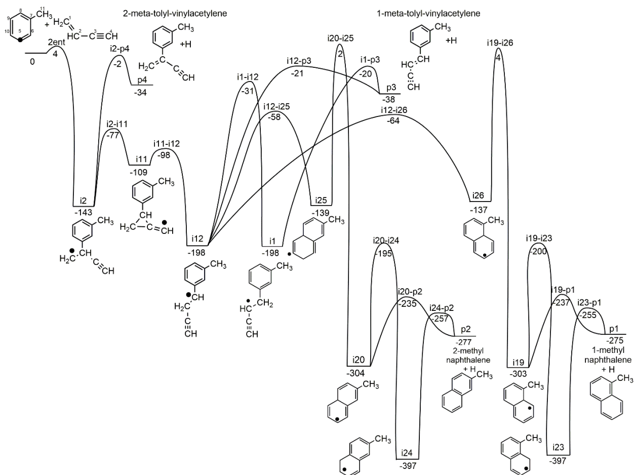
Figure 6. Proposed reaction mechanism based on stationary points on the C_{11}H_{11} potential energy surface for the reaction of the meta-tolyl radical with C2 carbon of vinylacetylene. Energies for intermediates, transition states, and products are given relative to the reactants energy (in \text{kJ mol}^{-1} ) at the at the UCCSD(T)-F12b/cc-pVDZ//UM06-2x/cc-pVTZ + ZPE(UM06-2x/cc-pVTZ) level of theory.
