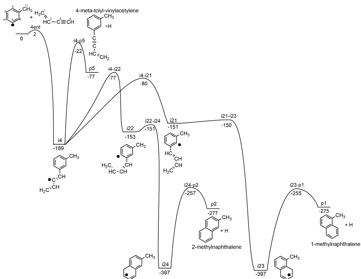
Figure 8. Proposed reaction mechanism based on stationary points on the C_{11}H_{11} potential energy surface for the reaction of the meta-tolyl radical with C4 carbon of vinylacetylene. Energies for intermediates, transition states, and products are given relative to the reactants energy (in \text{kJ mol}^{-1} ) at the at the UCCSD(T)-F12b/cc-pVDZ//UM06-2x/cc-pVTZ + ZPE(UM06-2x/cc-pVTZ) level of theory.
