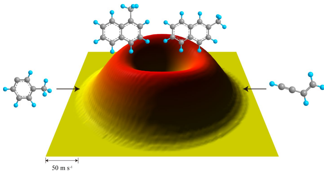
TOC Figure. Flux contour map for the reactive scattering channel of meta-tolyl radical with vinylacetylene.
