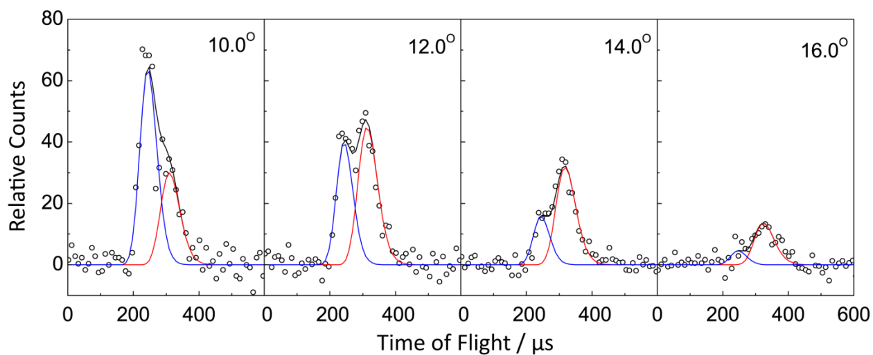
Figure 2. Selected time-of-flight (TOF) spectra recorded at a mass-to-charge ratio ( m/z ) of 142 for the reaction of meta-tolyl with vinylacetylene. The circles present the experimental data, the red and blue lines represent the fit for the reactive and non-reactive scattering channel, respectively. The black solid lines represent the overall fit.
