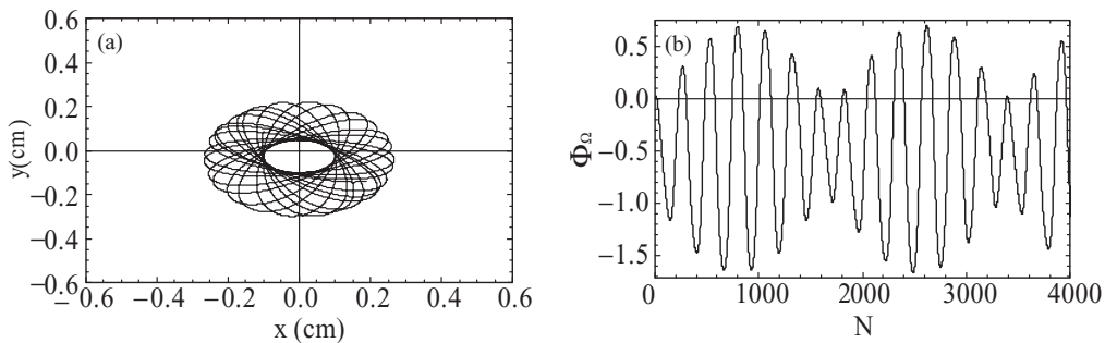
FIG. 4. (a) Simulated x - y trajectory of a particle as it moves N = 4000 twists = 100 m through the helical guide described in the text. (b) Accumulated geometric phase after a particle with the initial conditions described in the text travels from a uniform field region, through a helical guide of N turns, and exits into a second region of uniform field region.
