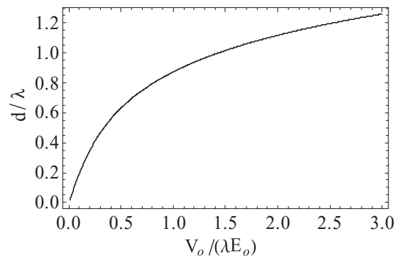
FIG. 2. Relationship between the d/\lambda and the V_o/(\lambda E_o) for the helical guide. Here voltages \pm V_o are placed on the electrodes, d is the inner diameter of the guide, \lambda = 2\pi/k is the pitch length, and E_o is the bias field of the guide.
