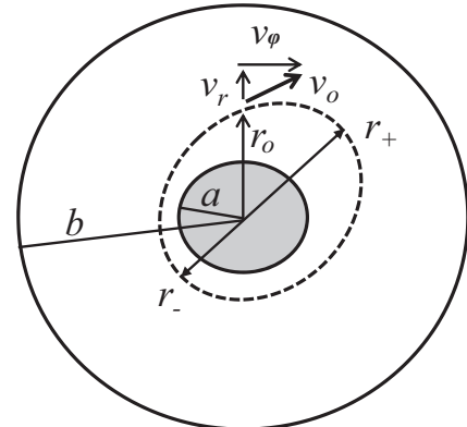
FIG. 5. Cross section of the cylindrical guide.
