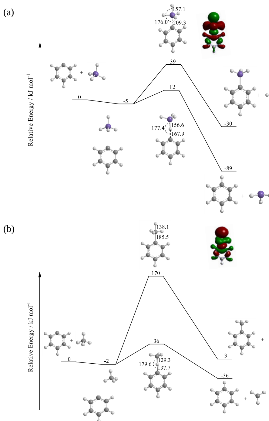
Fig. 3. Potential energy surfaces (PESs) in kJ mol -1 for the reactions of the phenyl radical with silane (a) and methane (b), respectively. Bond lengths and bond angles are given in pm and degrees, respectively. The highest occupied molecular orbital (HOMO) of the substitution transition states are also shown. Structures along with the vibrational frequencies of the reactants, intermediates, products, and transition states are compiled in the Supplementary Material (Table S1).
